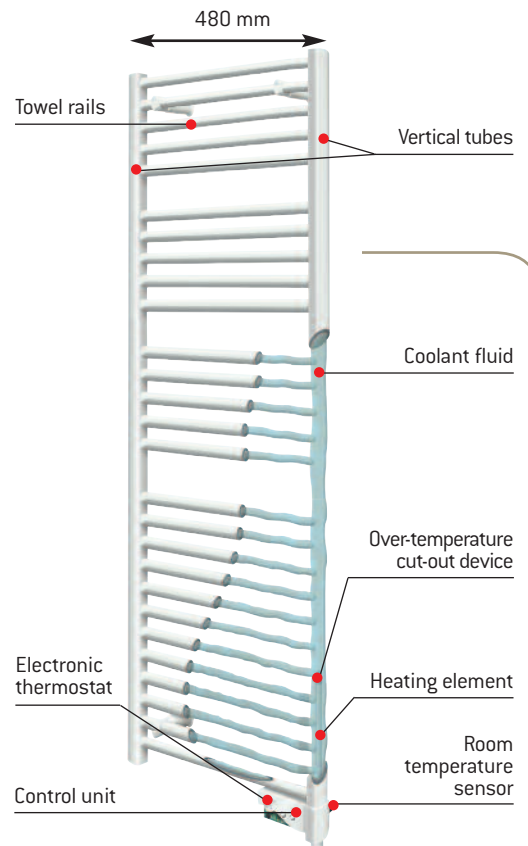
Control Unit
