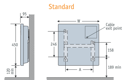
Front view showing bracket position.
